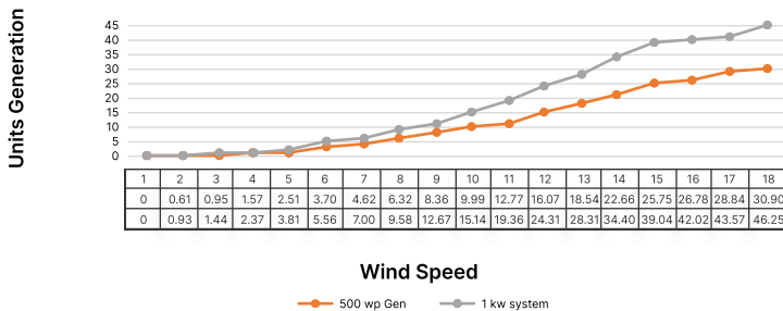
Power Curve Chart
