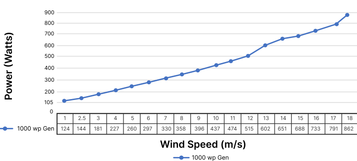
Power Curve Chart
